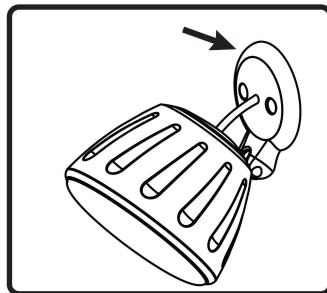
7. For outdoor installations, SoundTube recommends the use of marine-grade silicone caulk to seal around the area where the speaker meets the mounting surface. Failure to properly seal the mounting surface area may result in water ingress or damage.
