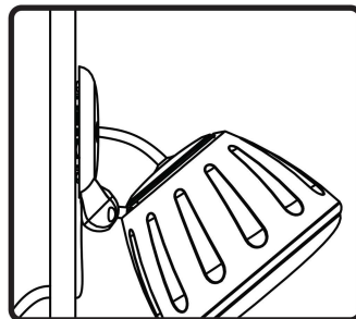
3b. If mounting speaker offset from wiring point, run wire out hole in wall and behind base plate through 2 mm standoff gap between base plate and wall. Standoff gap accepts up to 18-gauge flat signal wire.
