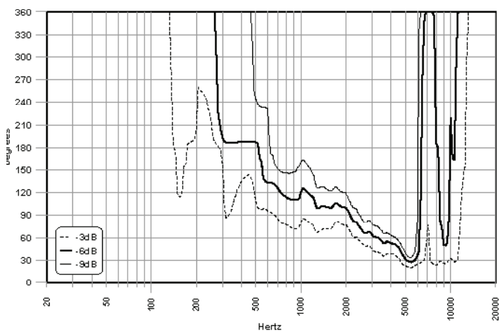
Vertical Beamwidth
