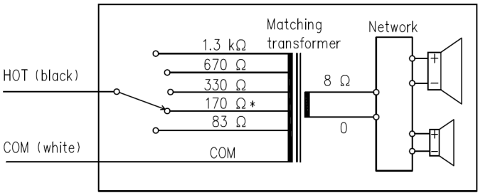
Wiring Diagram * Factory-preset
