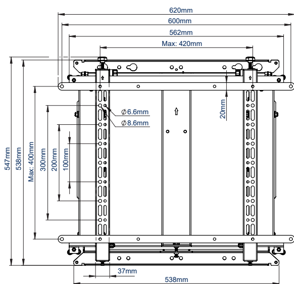
FRONT VIEW WITH ADAPTOR ARMS
