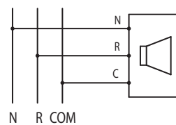
3-wire connection
