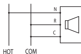
2-wire connection
