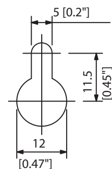
Fixing Hole (scale: 1/1)
