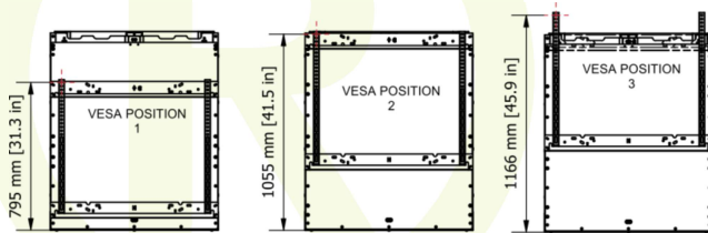
3 MOUNTING HEIGHTS FOR VESA 481A70
