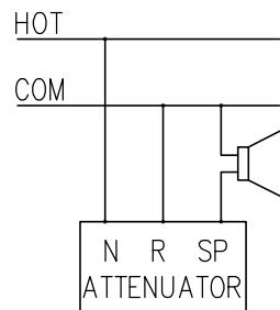
2-WIRE CONNECTION
