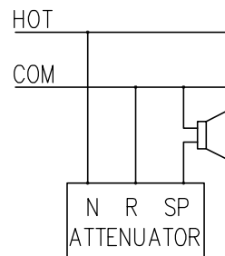
2-WIRE CONNECTION
