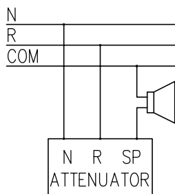
3-WIRE CONNECTION
